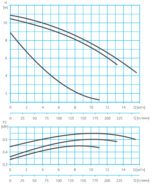
RA1-F 40-120
