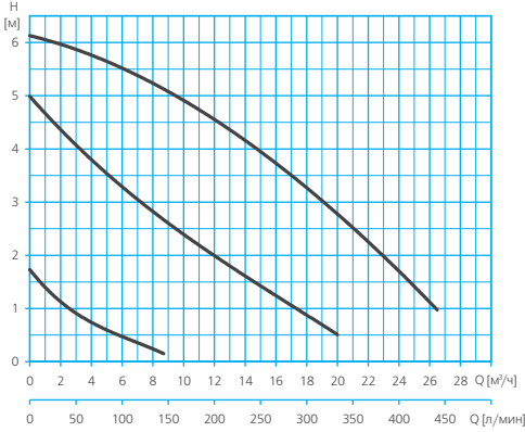
RA2-F 50-70 (3~400 V)
