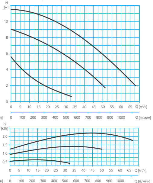
RA2-F 80-120 (3~400 V)
