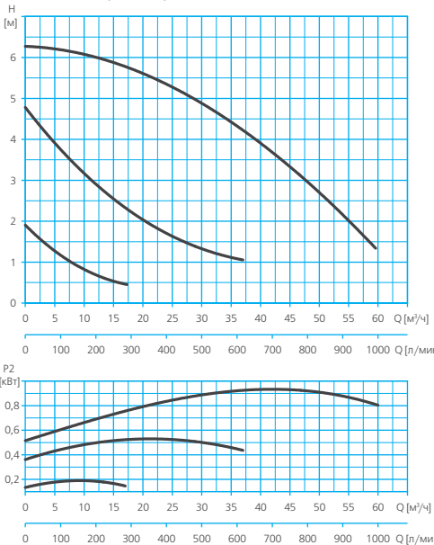
RA2-F 80-70 (3~400 V)
