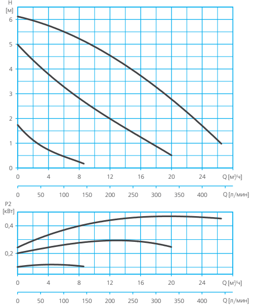
RA1-F 50-70 (3~400 V)
