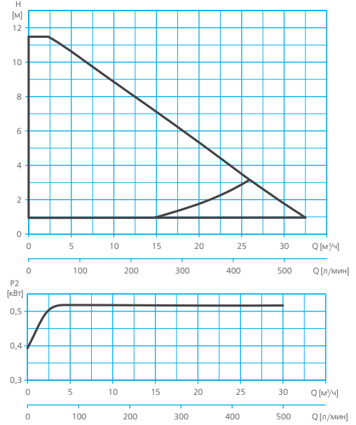
NMTD 40
