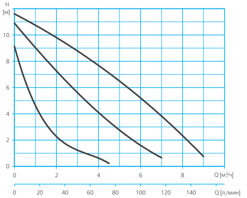
RA1-S 32-120-180
