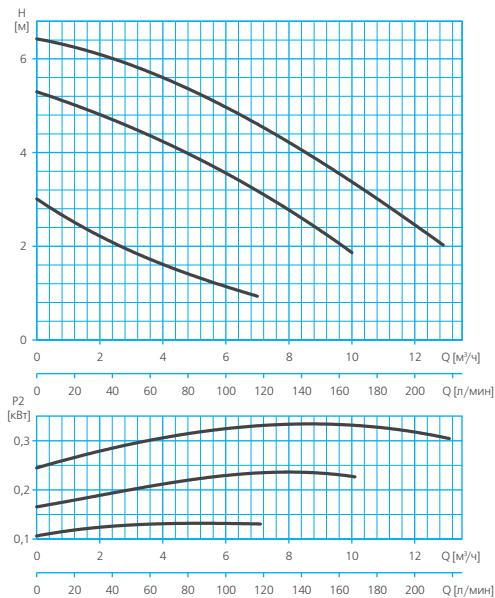
RSAN-F 40-70
