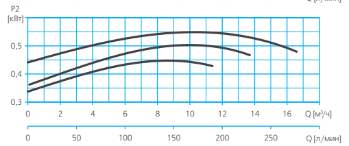
RA1-F 40-40 (3~400 V)
