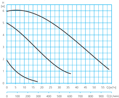
RA1-F 80-70 (3~400 V)
