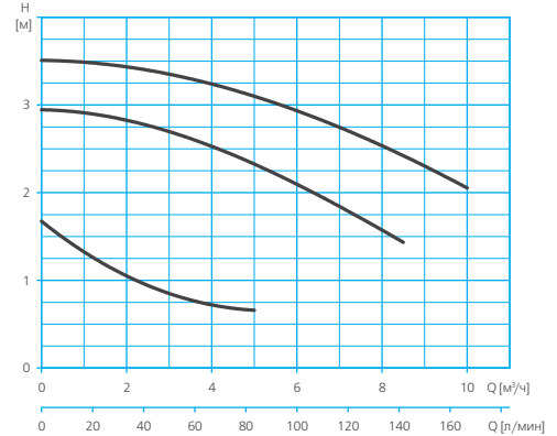
RA1-F 40-40 (3~400 V)
