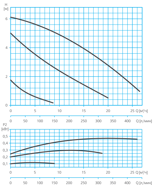
RSAN-F 50-70
